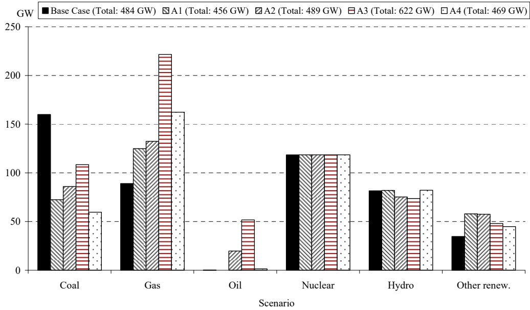
Figure 3. Maintained capacity of electricity generation by technologies under different allocation mechanisms. Case Common. GW
