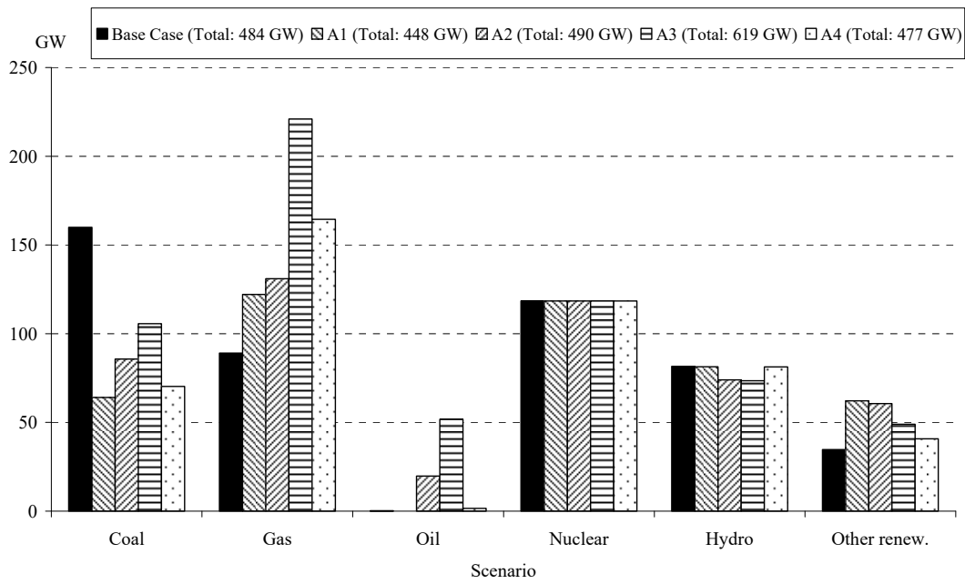
Figure 3. Maintained capacity of electricity generation by technologies under different allocation mechanisms. Case Common. GW
