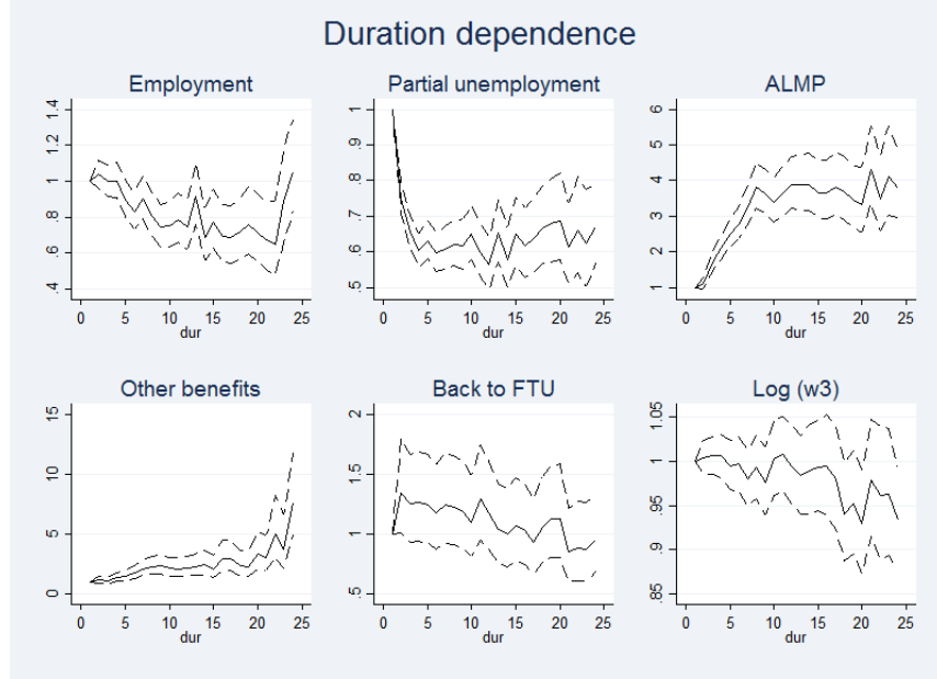
Figure 3: Model transitions
